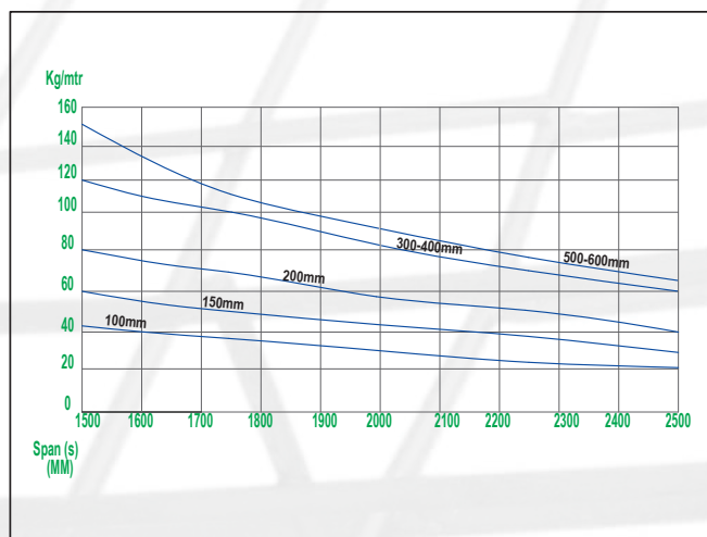
100mm Cable Basket
