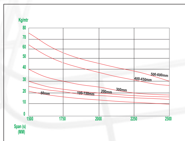
50mm Cable Basket
